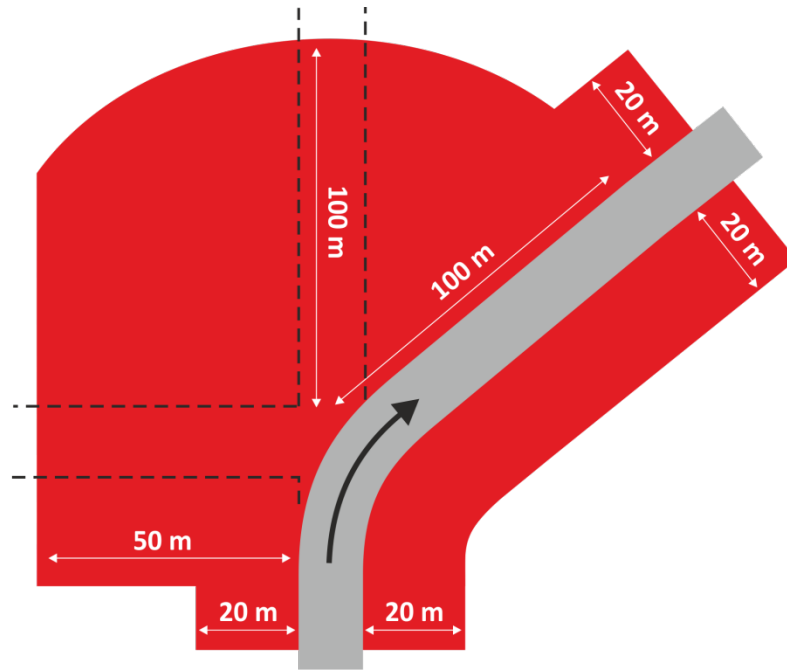
Turn of angle greater than 90° (intersection)
