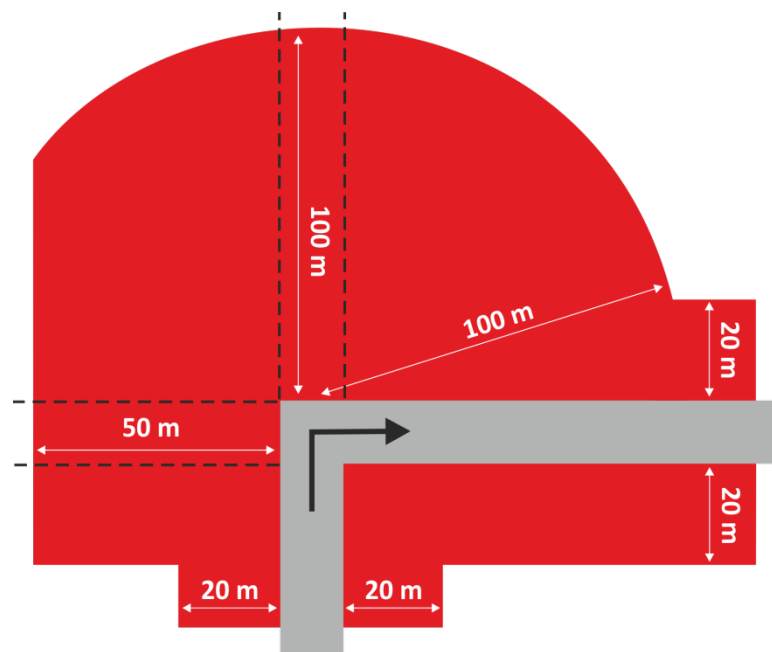
Turn of 90° or less (intersection)
