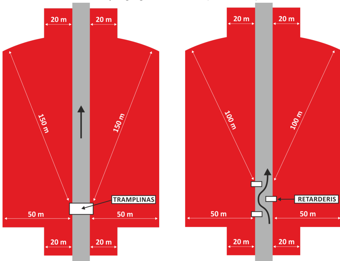
Jump and retarder on a straight section of the track
